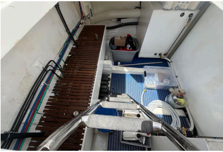
Engine room of 2006 Ocean Alexander 48 Classicco yacht with organized tools and equipment.
