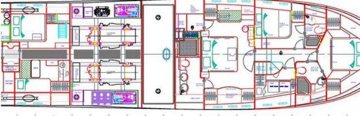
Blueprint of 2018 Marlow 75E-CB yacht, showcasing detailed interior and deck layout.
